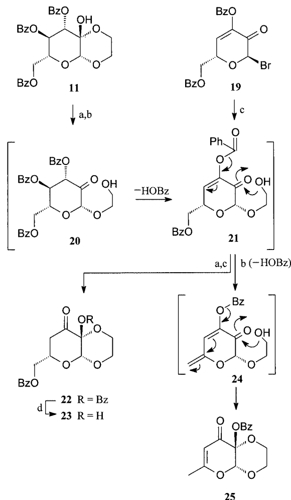
Scheme 4. Reagents and conditions: (a) \text{Bu}_4\text{NOAc} , \text{CH}_2\text{Cl}_2 , 1.5 h, room temperature, \rightarrow 22 (72%); (b) \text{Bu}_4\text{NOAc} , MeCN, 30 min, room temperature, \rightarrow 22 (29%) and 25 (34%); (c) \text{Ag}_2\text{CO}_3 , glycol, \text{CH}_2\text{Cl}_2 , 2 h, room temperature, \rightarrow 22 (82%); (d) \text{K}_2\text{CO}_3 , MeOH, 15 min, room temperature, 75%
