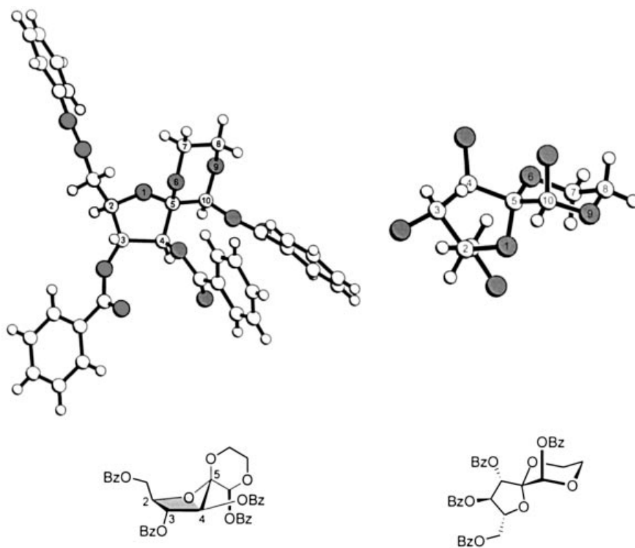
Figure 1. Perspective drawing and atomic numbering of 1,6,9-trioxaspiro[4,5]decane 30 as determined by X-ray crystallography; relevant dihedral angles around the spiro carbon (C-5): O1–C5–O6–C7 -63.6^\circ , O1–C5–C10–O9 +69.5^\circ , O1–C5–C10–O11 -167.7^\circ , O1–C5–C4–O40 -153.1^\circ [23]
