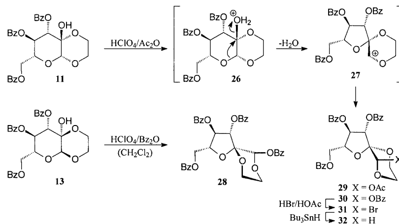
Scheme 5. Acid-induced pyranoid ring contraction of trioxadecalins 11 and 13 to trioxaspiro[4,5]decanes
